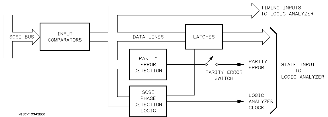
Figure 3-3. HP E2423A Block Diagram
