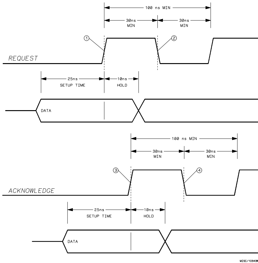
Figure 3-2. Request and Acknowledge Timing
