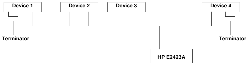
Figure 1-2. Connecting to the SCSI Bus
